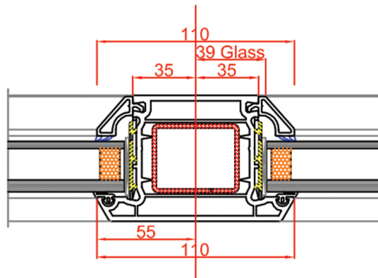
110mm Transom / Mullion Art no: 102.146
