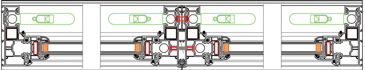
Coupling Art no: 116.005
