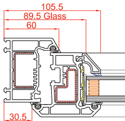
60mm Outer Frame Art no: 101.144 75mm Sash Art no: 103.150
