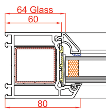
80mm Outer Frame Art no: 101.147
