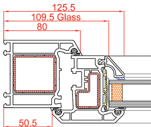
80mm Outer Frame Art no: 101.147 75mm Sash Art no: 103.150
