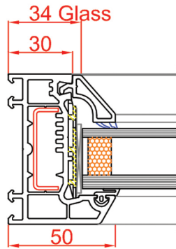
50mm Outer Frame Art no: 101.146
