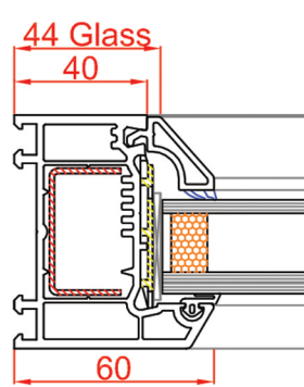
60mm Outer Frame Art no: 101.144
