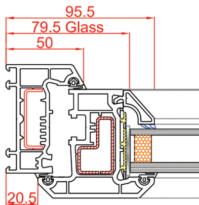
50mm Outer Frame Art no: 101.146 75mm Sash Art no: 103.150
